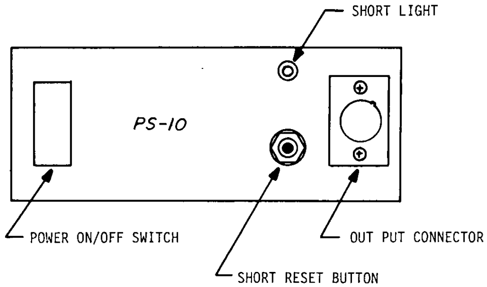
FRONT VIEW OF THE PS-10
