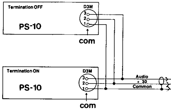
DUAL POWER SUPPLY INTERCONNECTION
