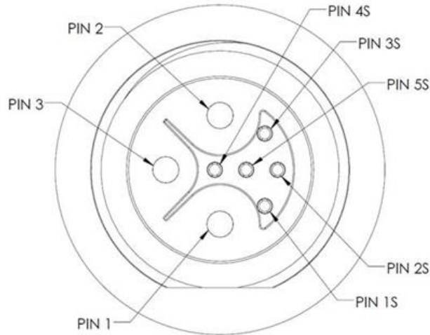
View of EXPLORER 122 Terminal Connector
